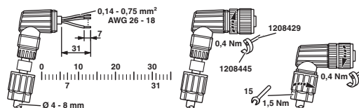
Functional drawing
