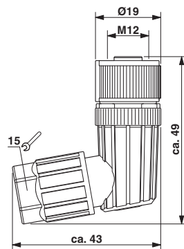
Dimensional drawing
